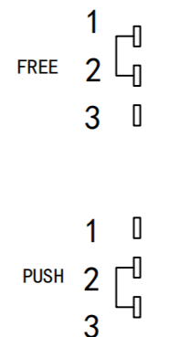
CIRCUIT DIAGRAM
