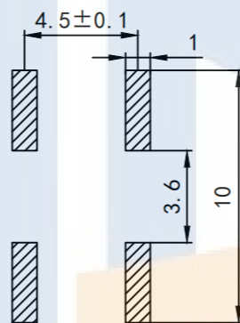
PWB land pattern for reference
