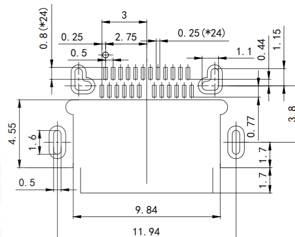
PECOMMENDED P. C. B. LAYOUT
