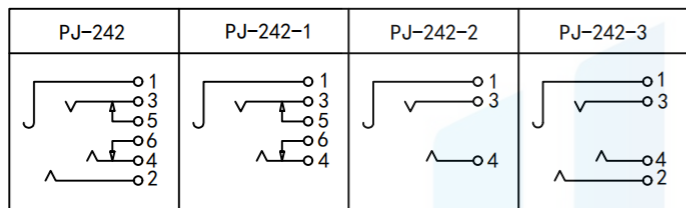
SCHEMATIC
