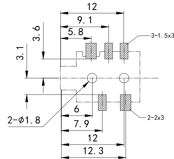
PCBLAYOUT
