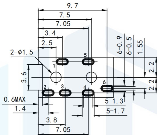
RECOMMEND PCB LAYOUT TOLERANCE: ±0.05
